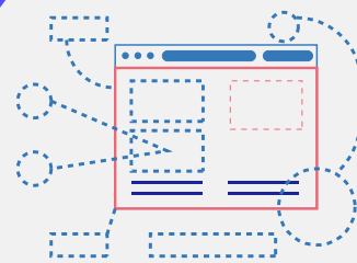
Webpage Structure
