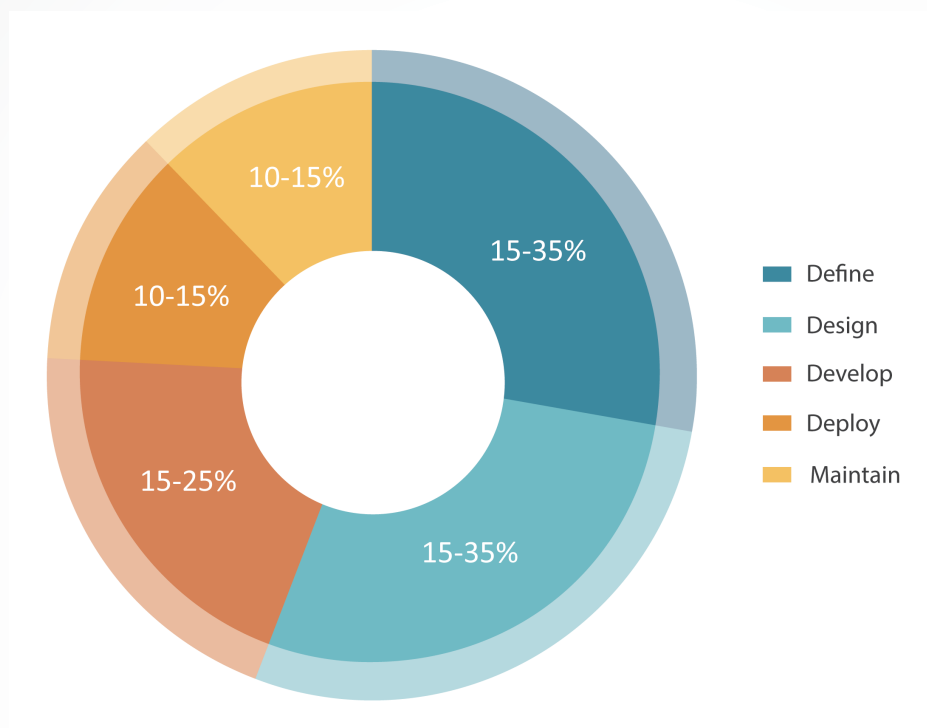
Figure 4 - Security test efforts proposed by OWASP in proportion to software development cycle
