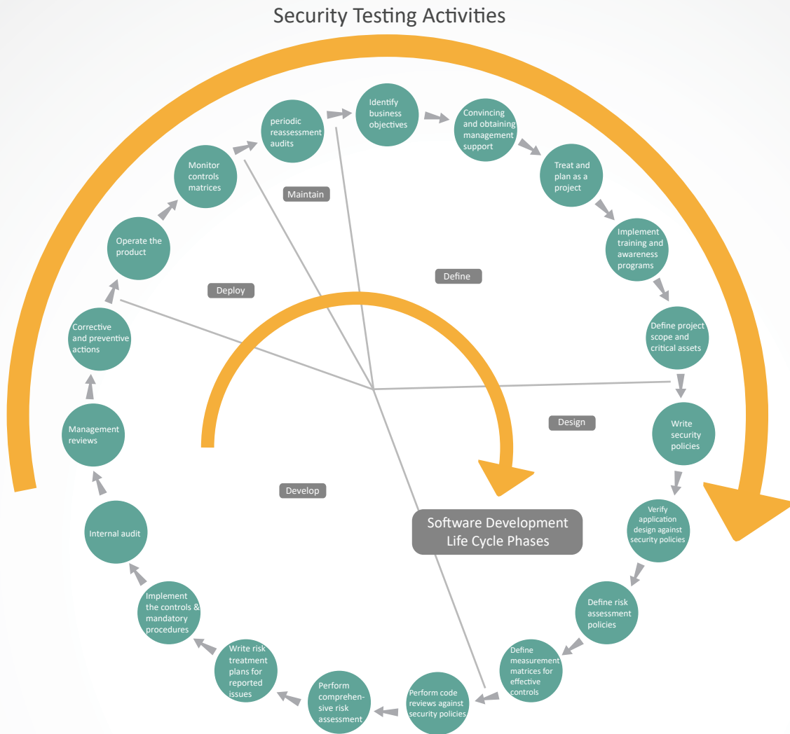
Figure 2 - Application security project activities aligned with Software development life cycle
